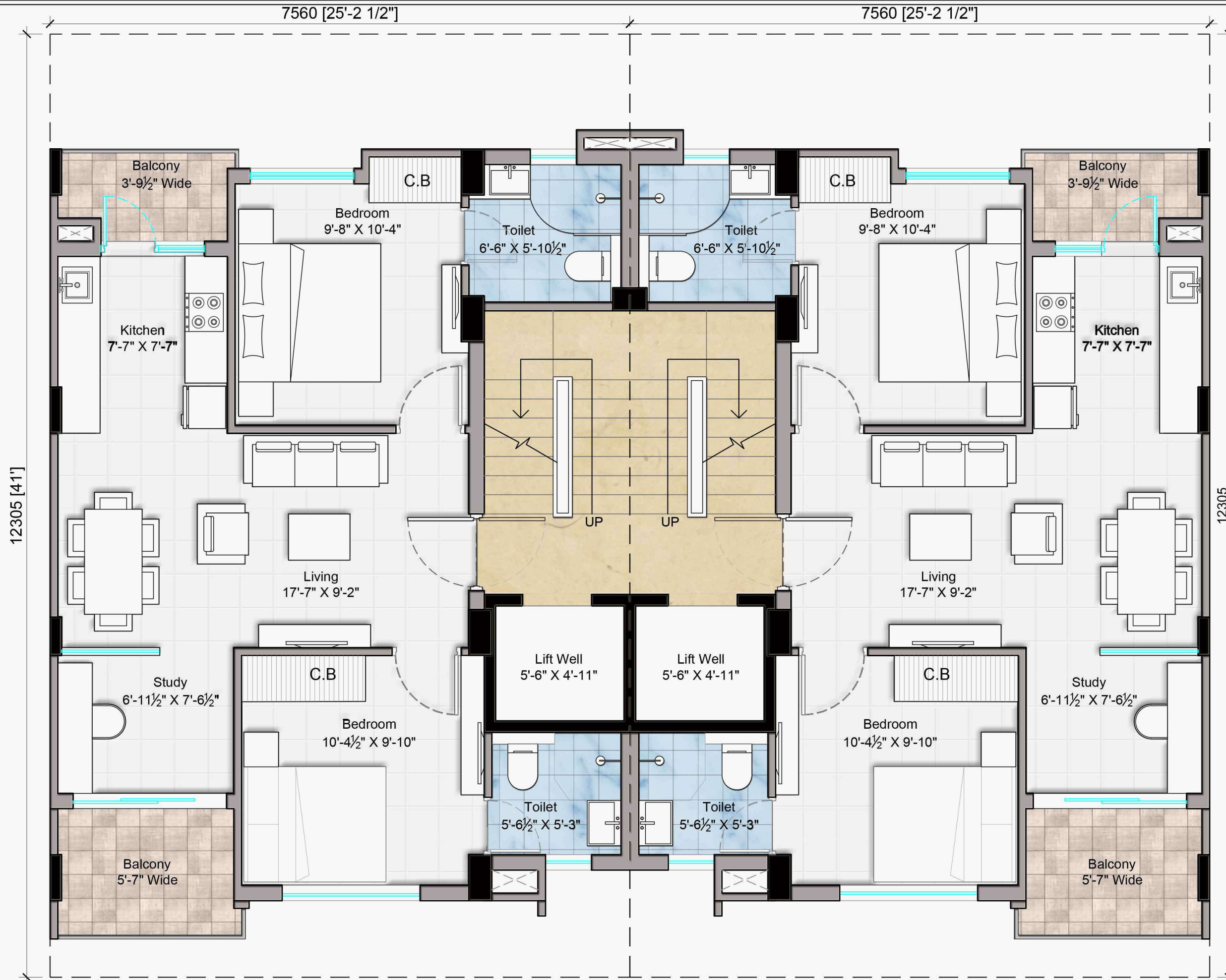
TYPICAL FLOOR LAYOUT
